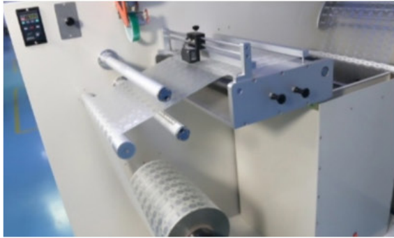
Antenna Unwinding
